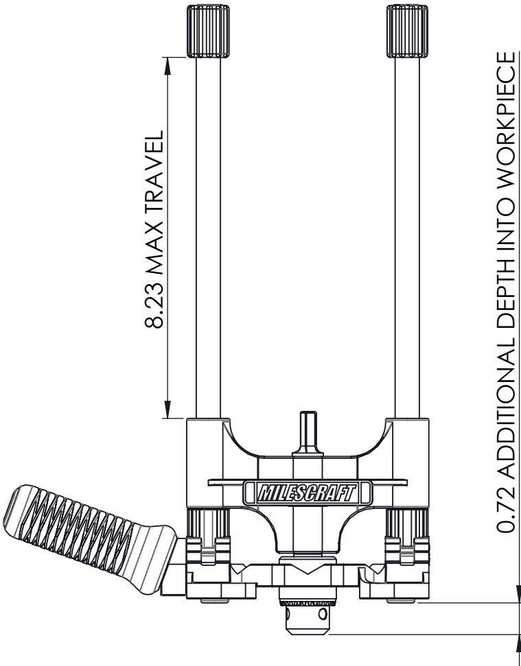
WITHOUT SPRING OR DEPTH STOP
